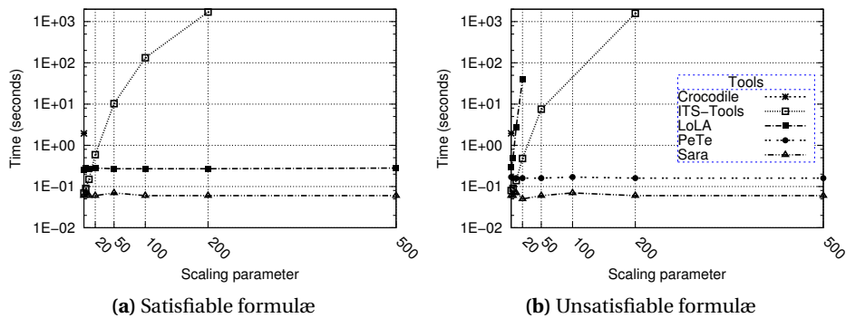
Fig. 7. Evolution of CPU consumption for reachability properties on FMS
